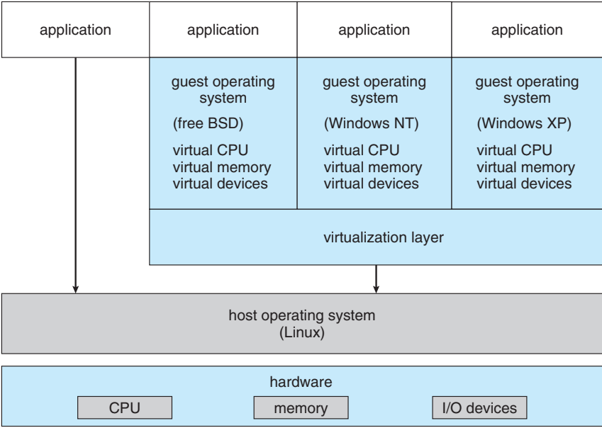
Figure 16.9 VMware Workstation architecture.
